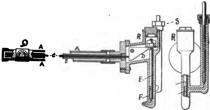
FIG. 211.—The White Thermostat Fuel Feed Regulator. A is a tube extending clear through the body of the steam generator and forming the connections of two of the coils, as at Q. B is a tube contained within A, and around which steam circulates; C, a rod contained within B; D, a bell crank regulating the valve, E, as C lengthens with heat; F, the point of the valve; R is the valve chamber, and S the gasoline inlet chamber regulated by a needle valve on a screw-threaded rod.
